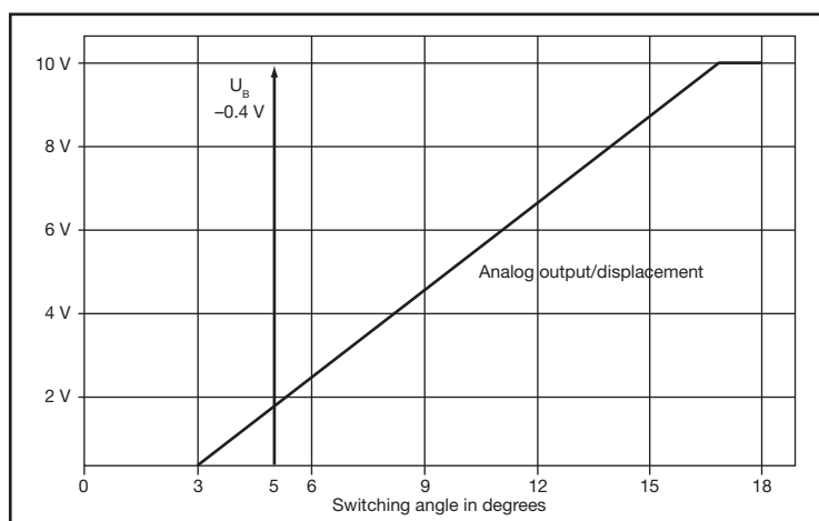
Voltage diagram
