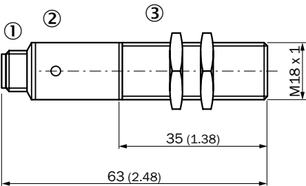
IMF18-xxBxxxxxx, M18, flush
