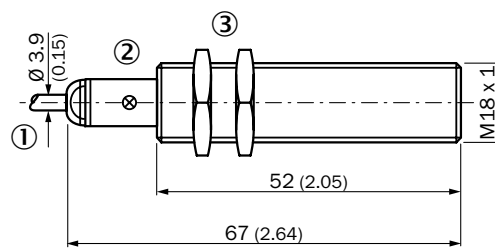
IME18-xxBxxxW2S, flush, cable, standard
