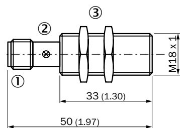
IME18-xxBxxxC0K, flush, connector, short-body housing
