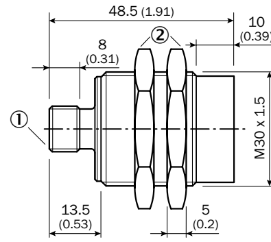
IMA30-xxNxxxCOK, M30, non-flush
