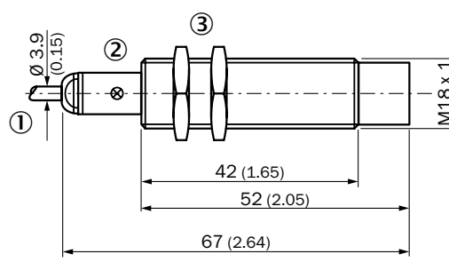
IME18-xxNxxxW2S, non-flush, cable, standard
