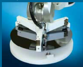
Wafer grippers of laser-formed material with SCHUNK Gripper LGP
