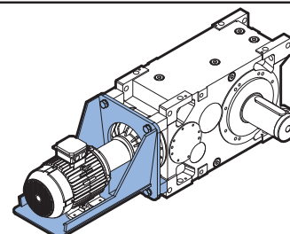
Motor Scoop (MC)
