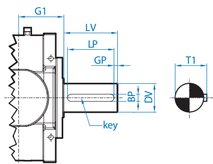
Solid Output Shaft
