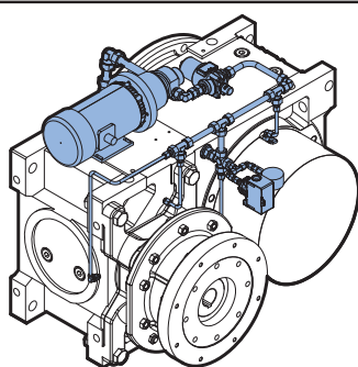
Pressure Forced Lubrication (LC) - Motor Driven
