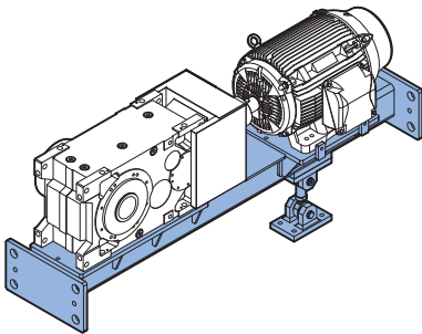
Motor Swing Base (MS) or Base Frame (MF)
