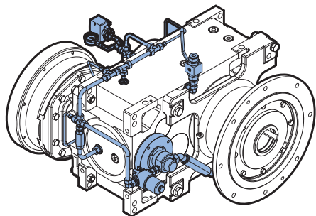
Pressure Forced Lubrication (LCX) - Shaft Driven
