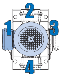
Right-Angle Gear Unit Terminal Box Positions *
