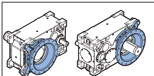
High output flange (FK) (B5 Flange with through holes)
