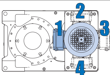
Parallel Gear Unit Terminal Box Positions *
