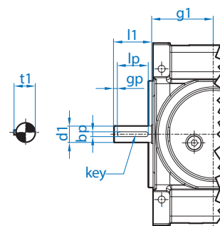
Solid Input Shaft
