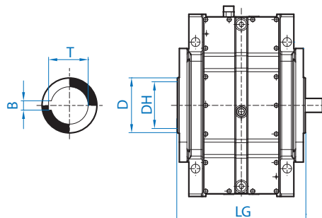
Hollow Shaft
