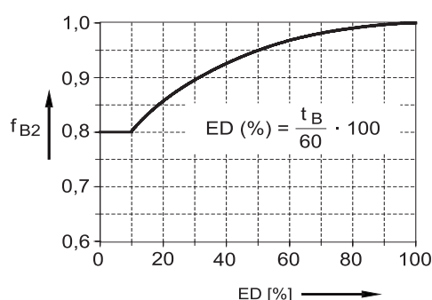
Diagram 3: Operating factor f_{B2} ED = Duration of switch-on t_B = Load time in min/h
