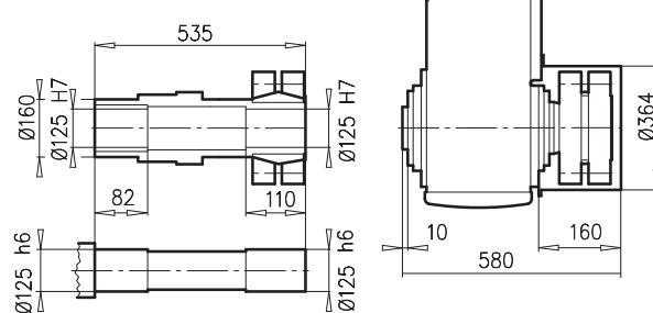
SK 9282ASH ⇨ A22
