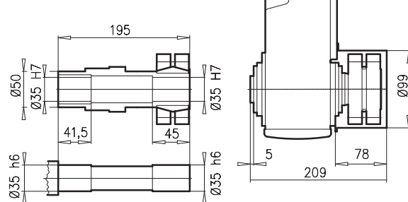
SK 2282ASH ⇨ A22
