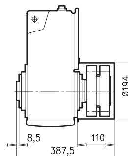
SK 6382ASH ⇨ A22
