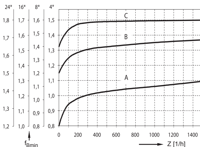
Diagram 1: Minimum operating factor f_{Bmin}
